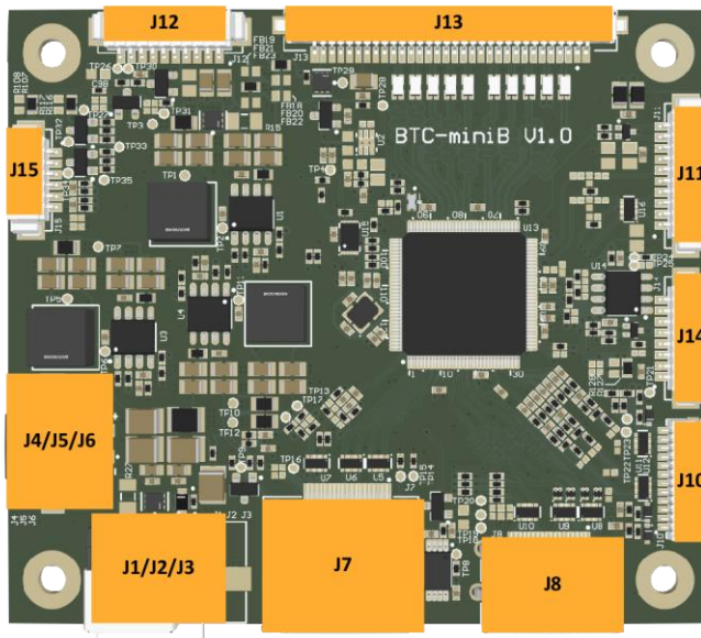
Fig 6. Connector Overview
