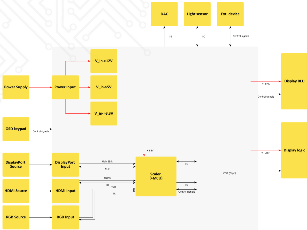
Fig 1. System Diagram
